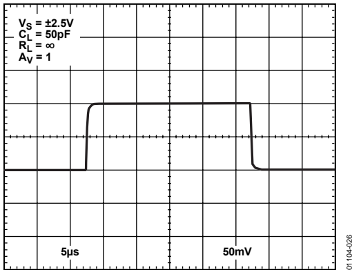
Figure 26. Small Signal Transient Response at 5 V
