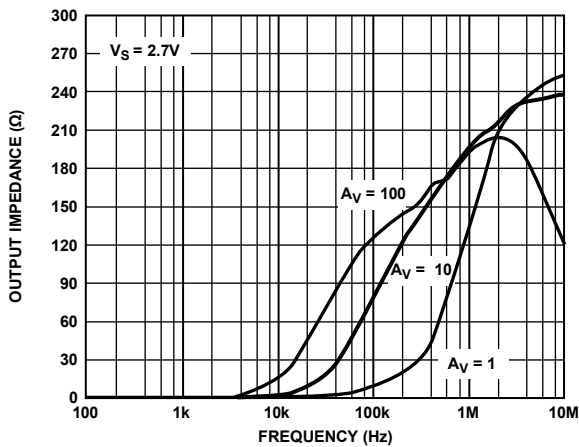
Figure 21. Output Impedance vs. Frequency at 2.7 V
