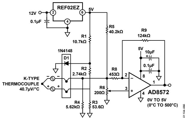
Figure 66. Precision K-Type Thermocouple Amplifier with Cold-Junction Compensation
