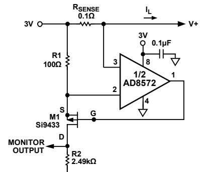
Figure 67. High-Side Load Current Monitor
