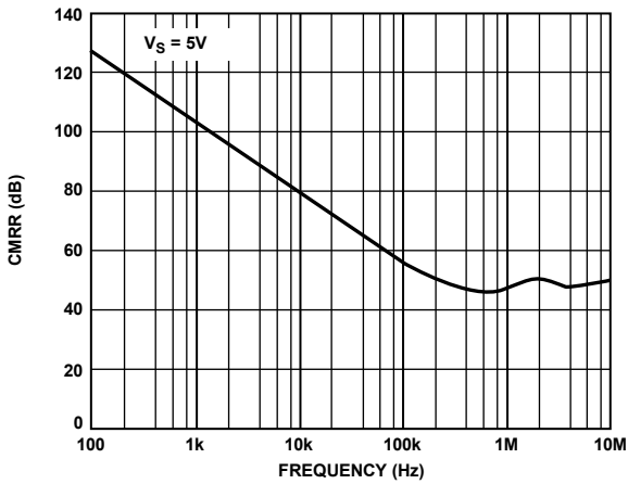
Figure 33. CMRR vs. Frequency at 5 V
