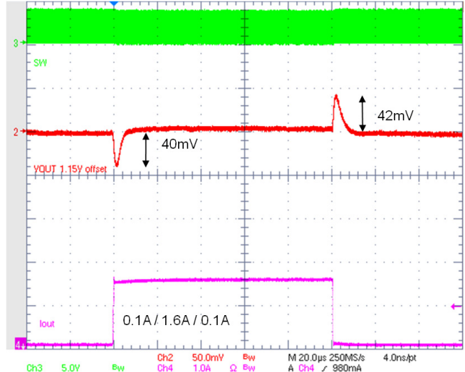
Figure 29. Transient Load 0.1 – 1.6 A Forced PWM Mode
