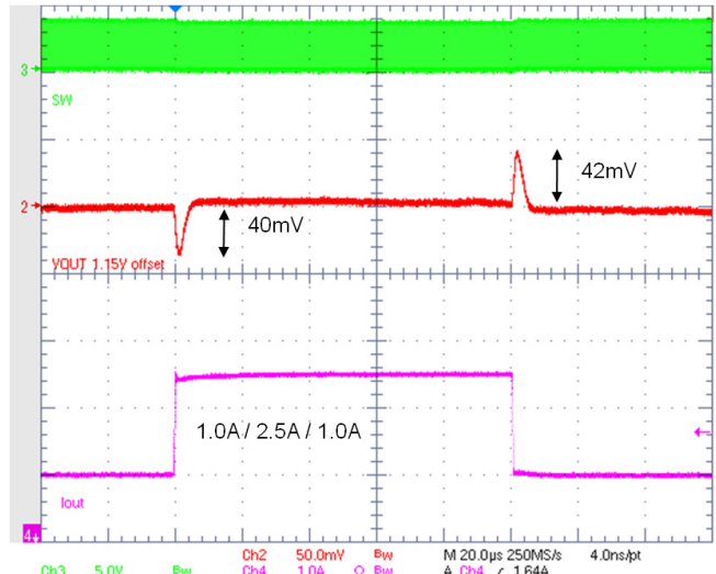
Figure 31. Transient Load 1.0 – 2.5 A Forced PWM Mode
