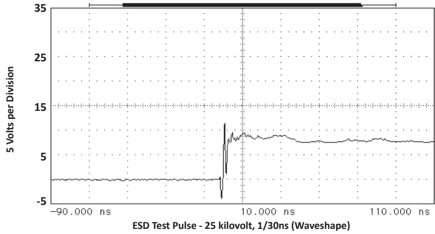
FIGURE 4 OVERSHOOT & CLAMPING VOLTAGE FOR U0402FC05C
