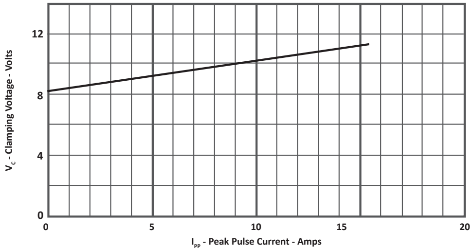
FIGURE 5 TYPICAL CLAMPING VOLTAGE VS PEAK PULSE CURRENT U0402FC05C
